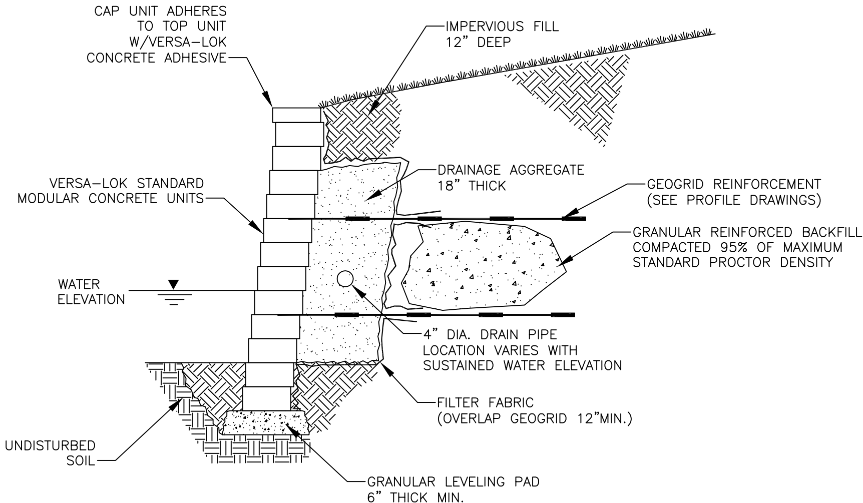
TYPICAL SECTION—REINFORCED RETENTION POND WALL SCALE: NONE
